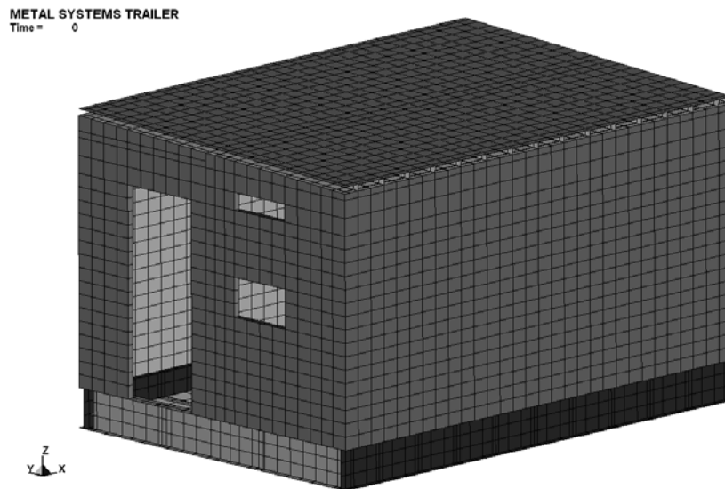
Figure 3 - Half-Symmetry Building Model
