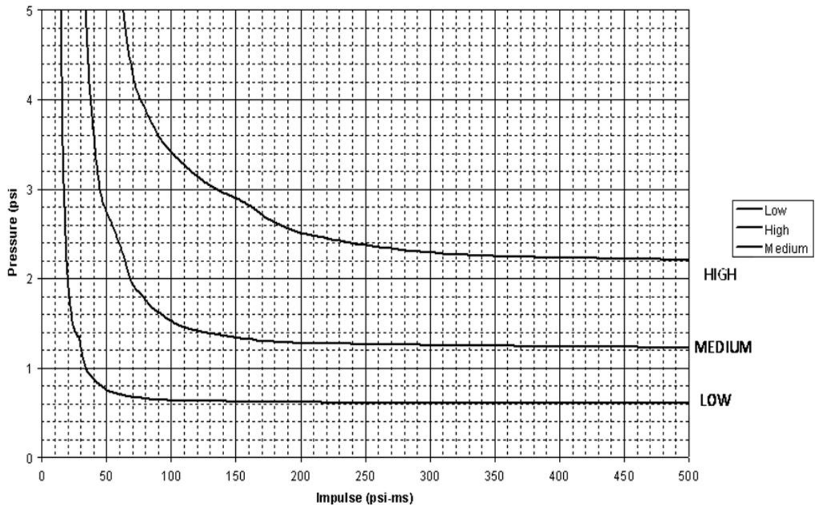
Figure 2 - Side-On Pressure-Impulse Diagram for 2.7 mm Wall Panels
