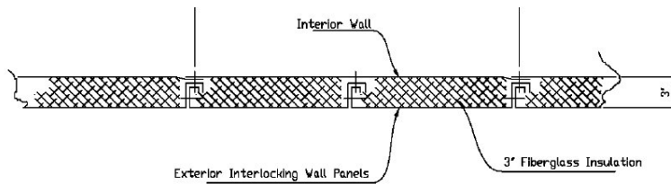
Figure 4 - Typical Interlocking Wall Panel Section
